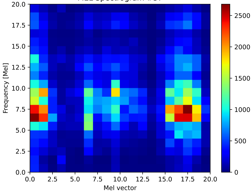
MEL Spectrogram #37
